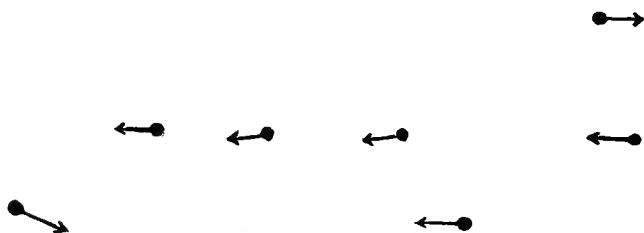
THE "GREAT DIPPER" AS IT IS
